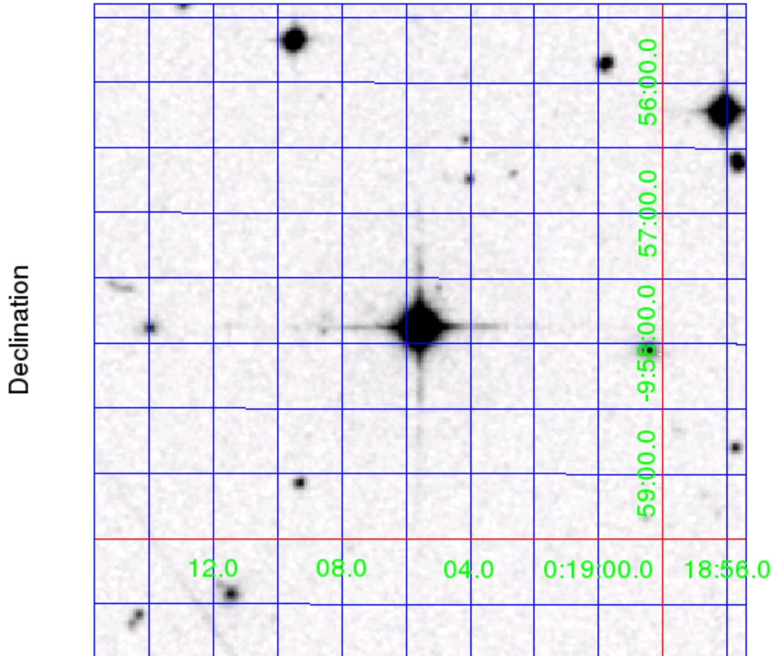
Digitized Sky Survey (DSS) red image. The 5' x 5' image is centered on the J2000 coordinates of target (37749396).
