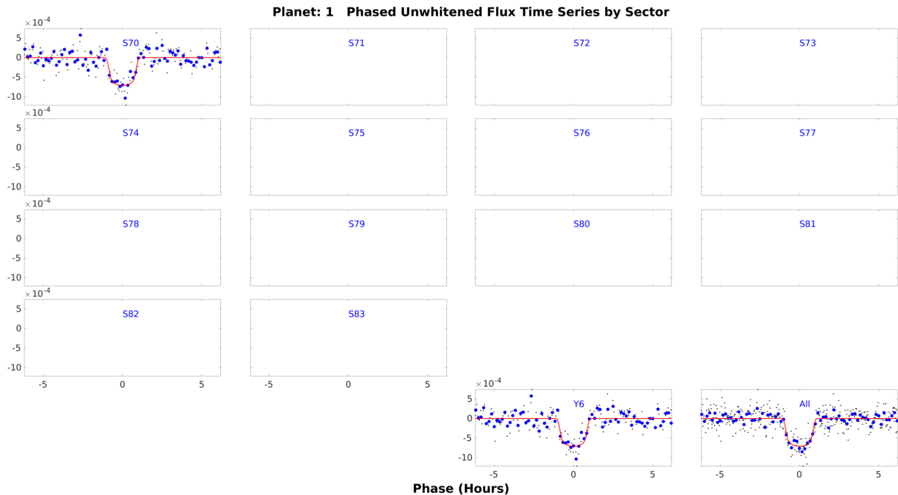
Phased unwhitened flux time series by sector in year 6 for target 37749396, planet candidate 1. Period = 13.4758 days; transit epoch = 1392.294 BTJD. Open ./summary-plots/0000000037749396-01-phased-unwhitened-flux-time-series-by-sector-06.fig
