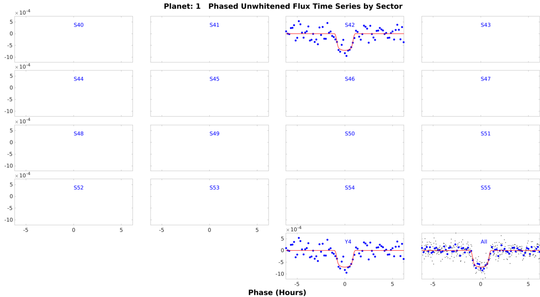
Phased unwhitened flux time series by sector in year 4 for target 37749396, planet candidate 1. Period = 13.4758 days; transit epoch = 1392.294 BTJD. Open ./summary-plots/0000000037749396-01-phased-unwhitened-flux-time-series-by-sector-04.fig
