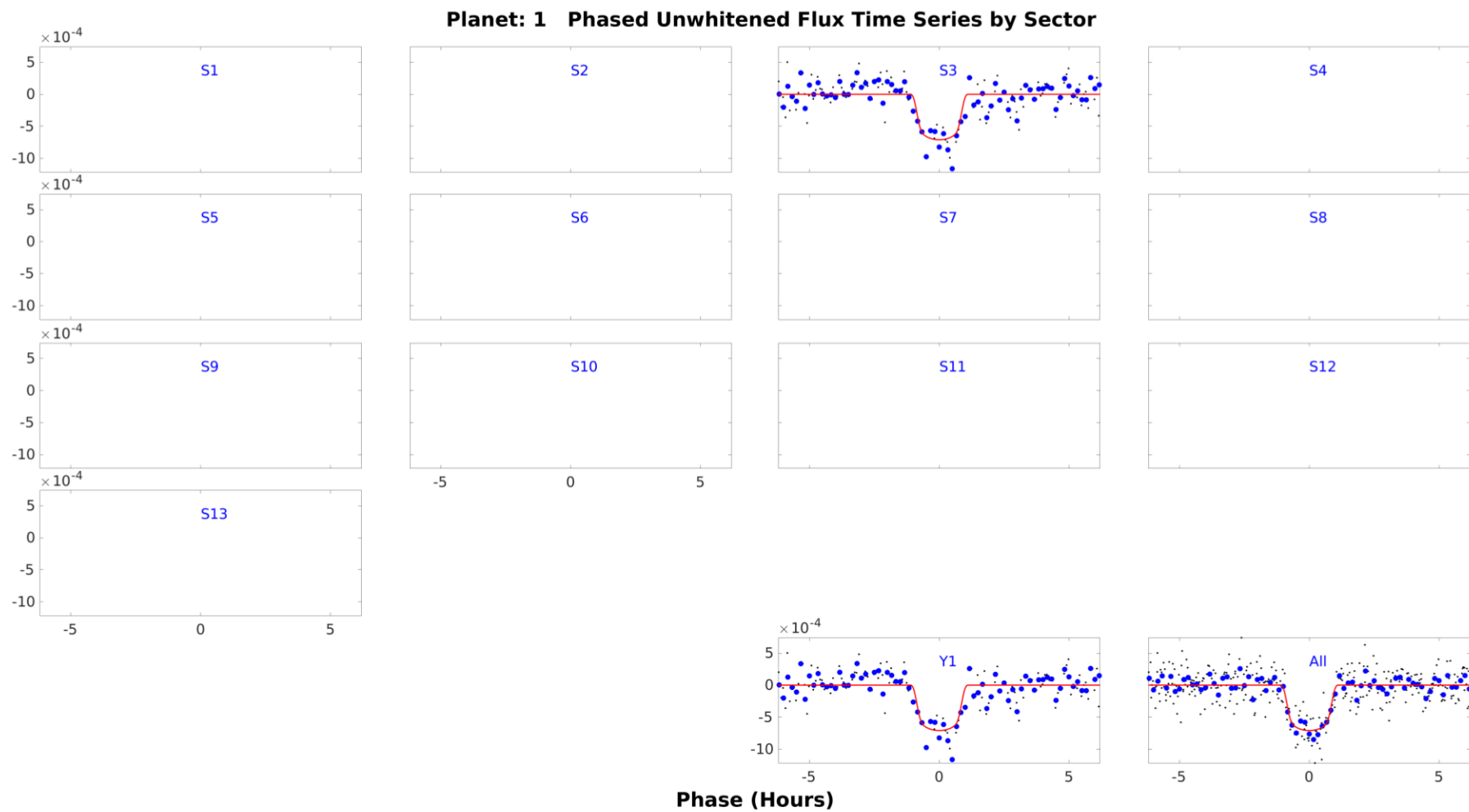
Phased unwhitened flux time series by sector in year 1 for target 37749396, planet candidate 1. Period = 13.4758 days; transit epoch = 1392.294 BTJD. Open ./summary-plots/0000000037749396-01-phased-unwhitened-flux-time-series-by-sector-01.fig
