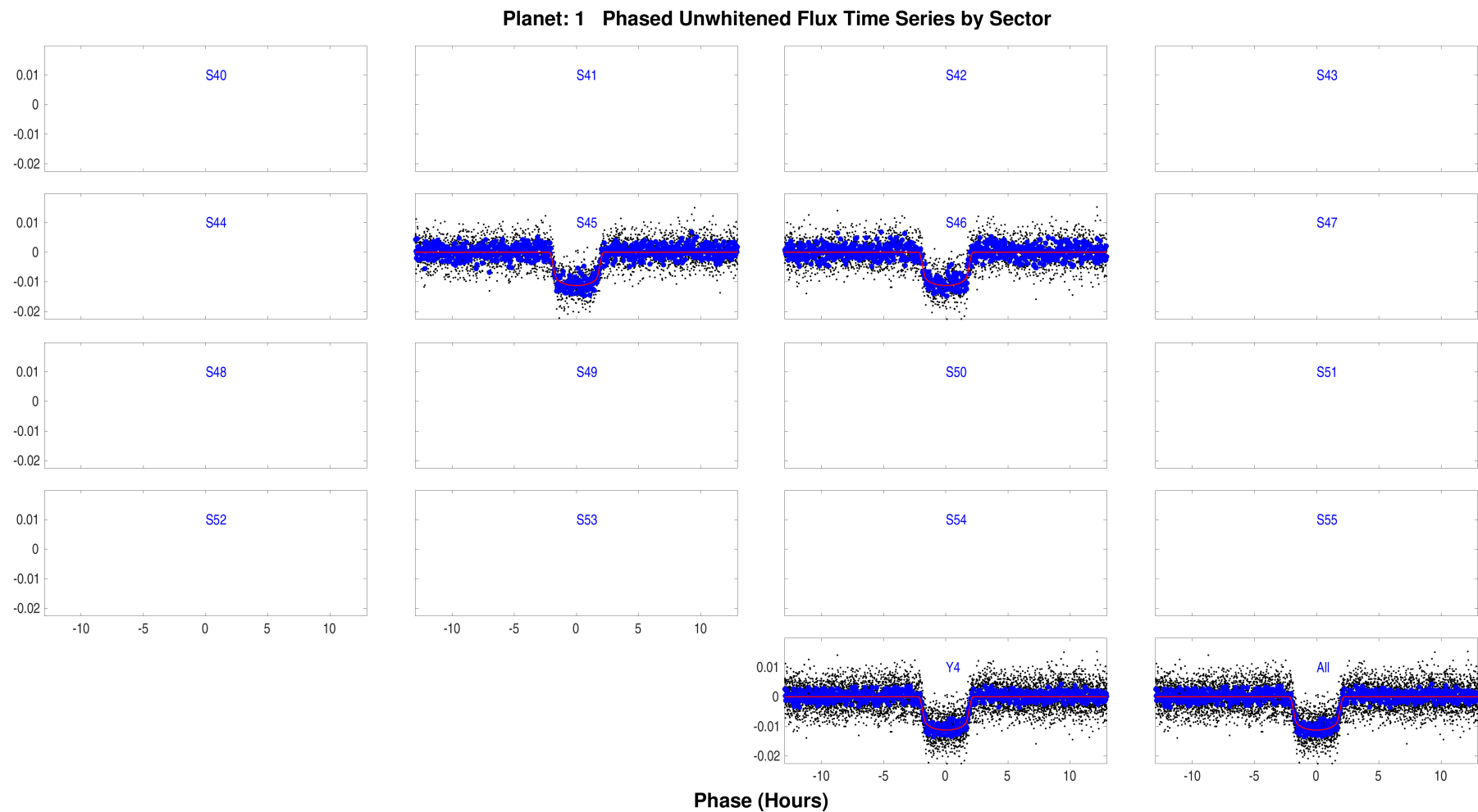
Phased unwhitened flux time series by sector in year 4 for target 169249234, planet candidate 1. Period = 7.1856 days; transit epoch = 2527.4325 BTJD. Open ./summary-plots/0000000169249234-01-phased-unwhitened-flux-time-series-by-sector-04.fig
