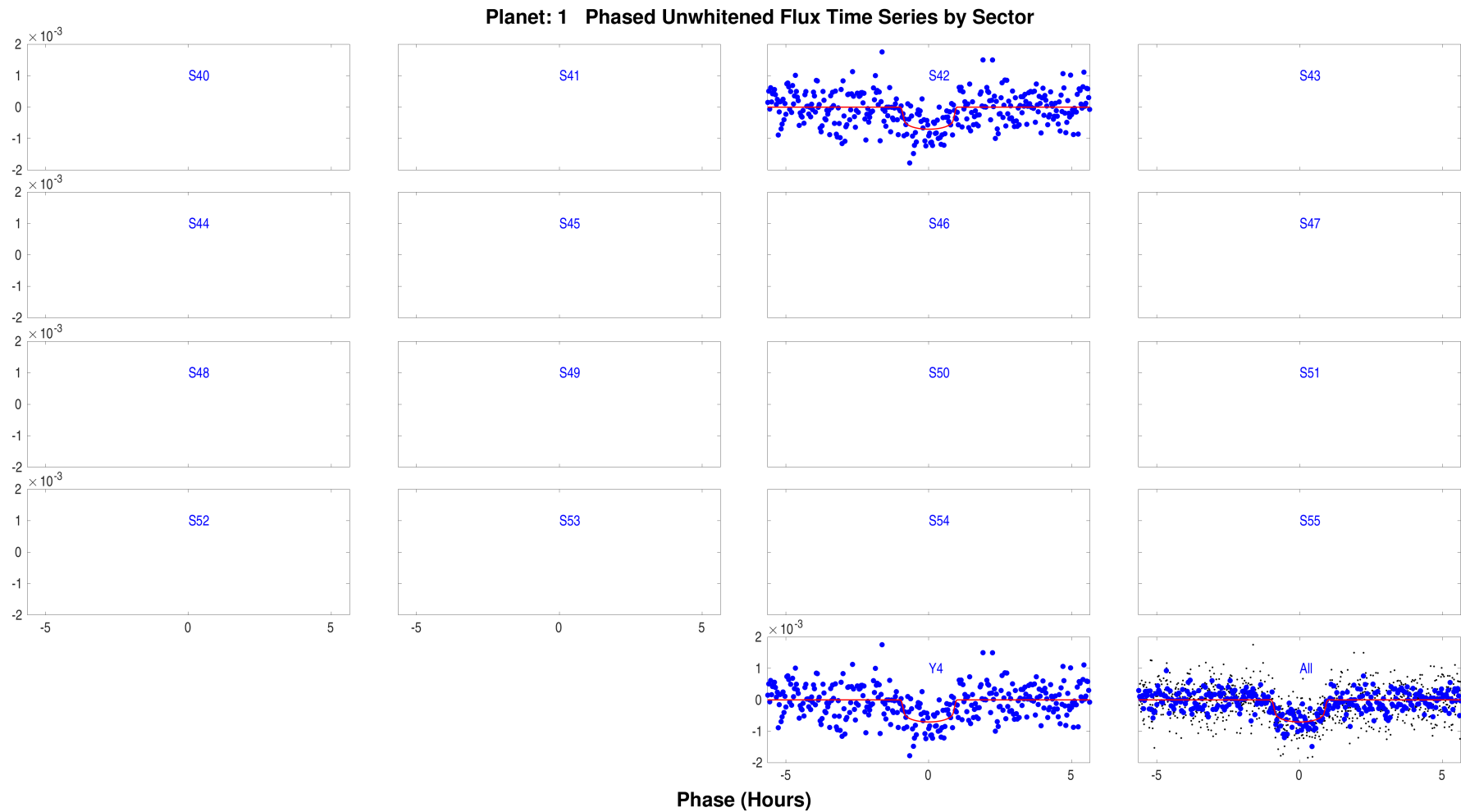
Phased unwhitened flux time series by sector in year 4 for target 37749396, planet candidate 1. Period = 13.4758 days; transit epoch = 1392.2938 BTJD. Open ./summary-plots/000000037749396-01-phased-unwhitened-flux-time-series-by-sector-04.fig
